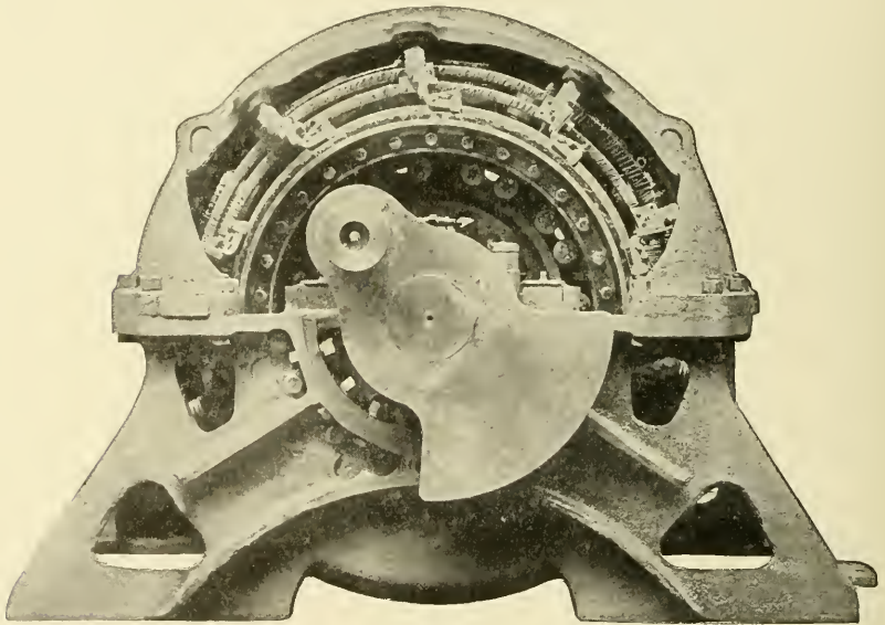
Fig. 252. Side View of Pennsylvania Locomotive Motor
